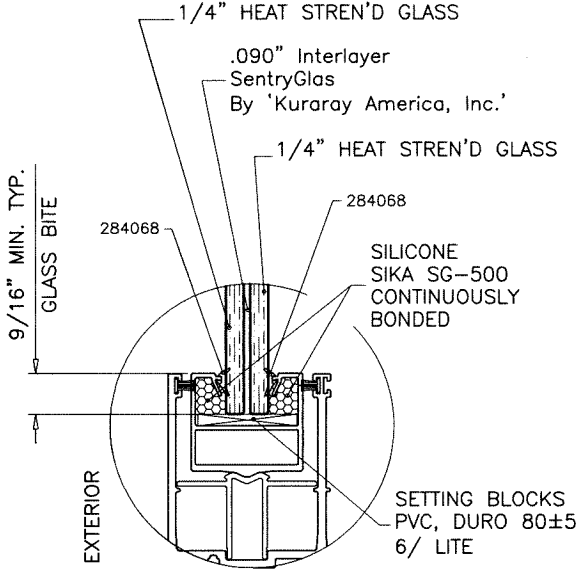
GLASS TYPE 'C' 9/16" OVERALL LAMINATED GLASS
