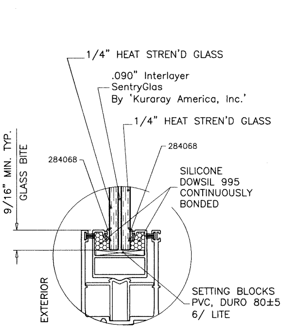
GLASS TYPE 'B' 9/16" OVERALL LAMINATED GLASS
